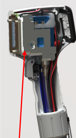
360 degree ring cooling plate
